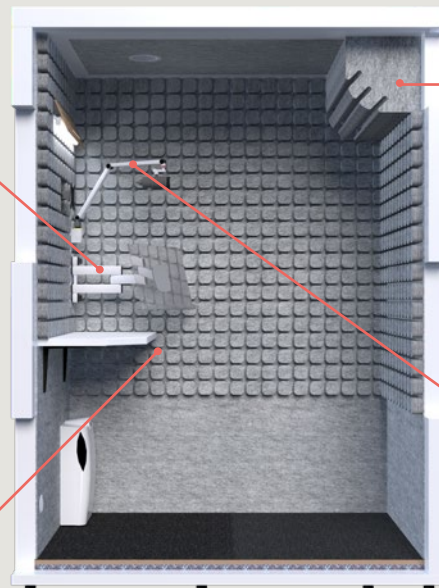
ACOUSTIC- ABSORBING PANELS ECO45 AT LEVEL D
